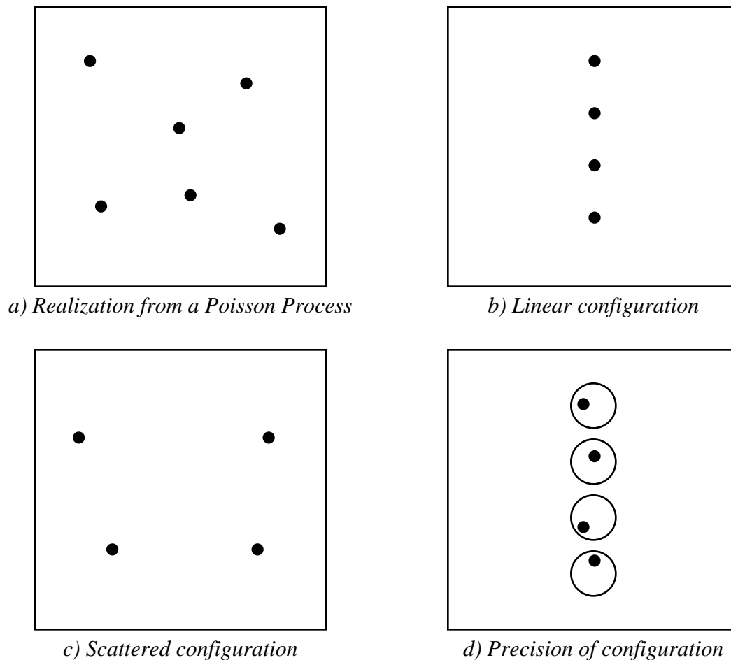
Figure D-1 Modeling configurations of point features as a Poisson process
